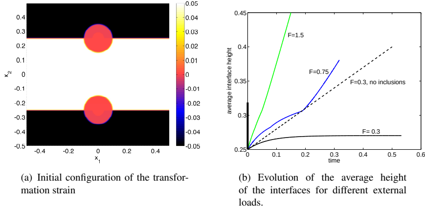
Fig. 1 Initial condition and evolution of the interface depending on the external load
